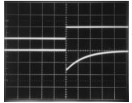
10µs/div A = OUTPUT CURRENT, 1mA/div, I_{OUT} = 0mA to 1mA B = OUTPUT VOLTAGE, 50mV/div
