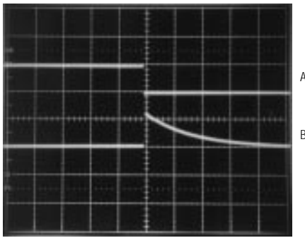
10µs/div A = OUTPUT CURRENT, 1mA/div, I_{OUT} = 0mA to -1mA B = OUTPUT VOLTAGE, 200mV/div
