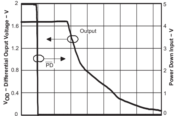
Figure 30. Turnoff Time
