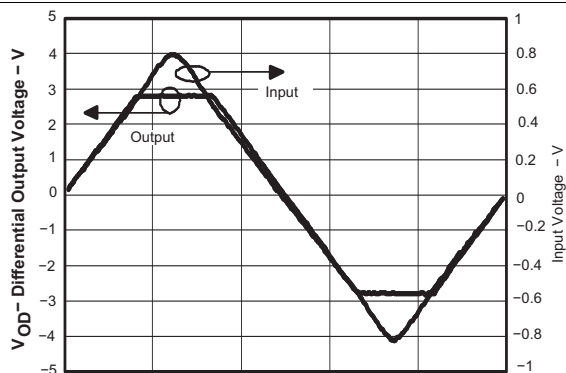
Figure 28. Overdrive Recovery
