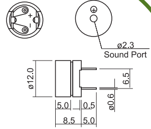
Dimension Unit: mm Tolerance : 0.3mm
